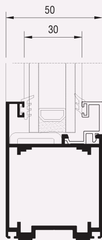
Double Glazed
