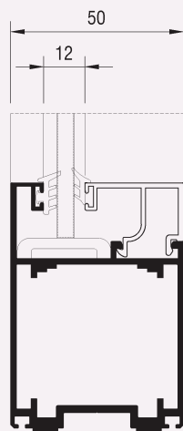
Single Glazed
