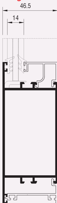
Single Glazed
