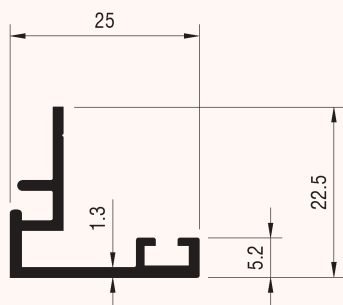
Profile Code : FD-6005 Unit Weight : 0.242 kg/m Perimeter : 137.5 mm
