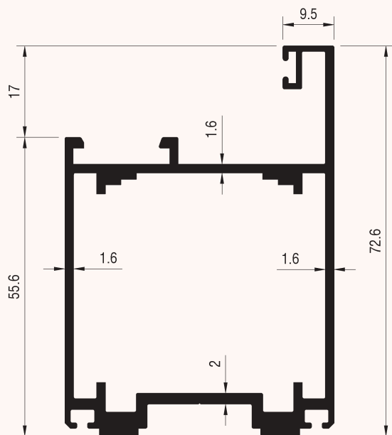
Profile Code : FD-6004 Unit Weight : 1.376 kg/m Perimeter : 342.9 mm
