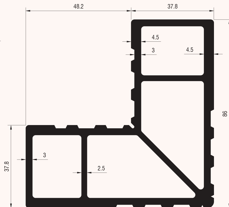
Profile Code : FD-6006 Unit Weight : 4.041 kg/m Perimeter : 370.0 mm
