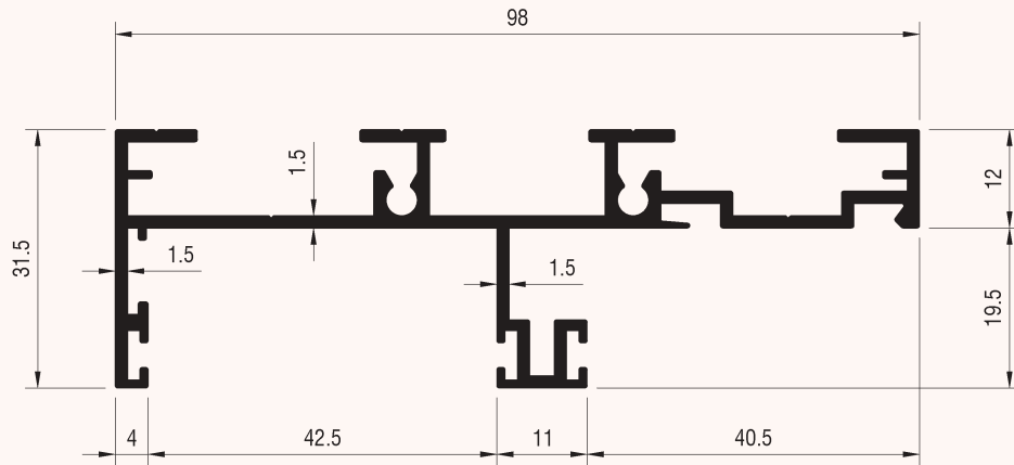
Profile Code : SD-1031 Unit Weight : 1.118 kg/m Perimeter : 554.3 mm
