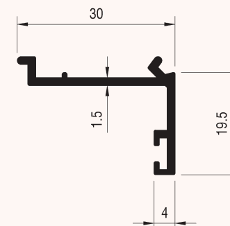
Profile Code : SD-1044 Unit Weight : 0.258 kg/m Perimeter : 130.1 mm
