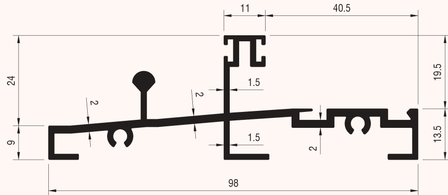
Profile Code : SD-1032 Unit Weight : 1.158 kg/m Perimeter : 485.9 mm
