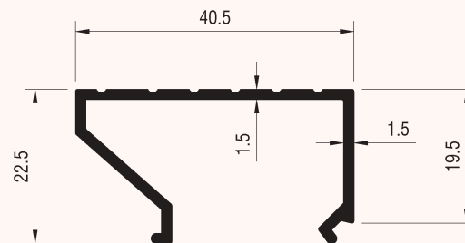
Profile Code : SD-1034 Unit Weight : 0.367 kg/m Perimeter : 187.8 mm
