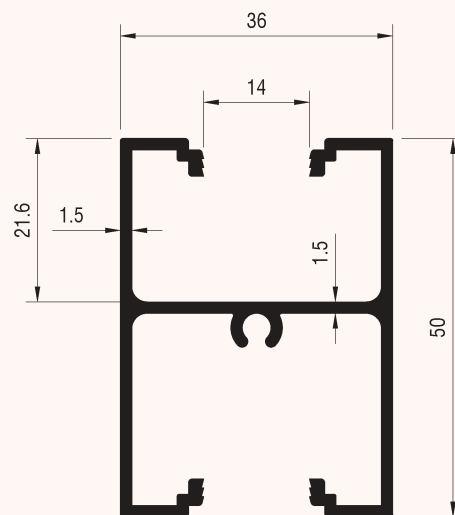
Profile Code : SD-1039 Unit Weight : 0.804 kg/m Perimeter : 384.3 mm
