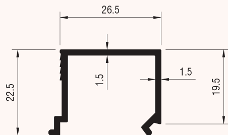
Profile Code : SD-1033 Unit Weight : 0.310 kg/m Perimeter : 151.0 mm
