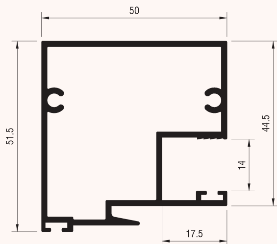
Profile Code : SD-1040 Unit Weight : 1.023 kg/m Perimeter : 278.4 mm
