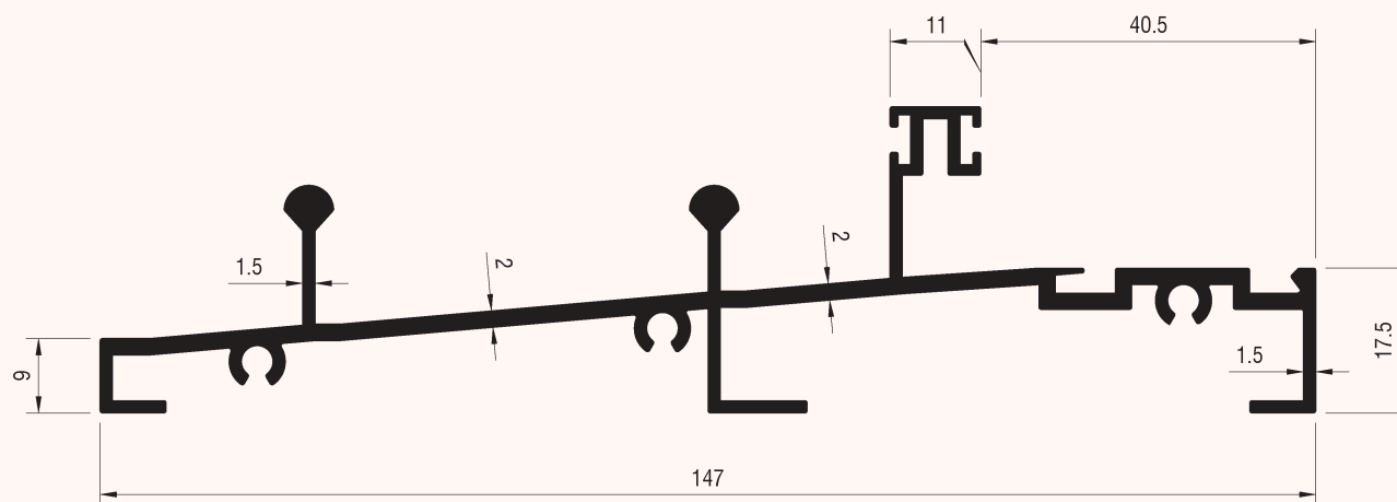
Profile Code : SD-1042 Unit Weight : 1.601 kg/m Perimeter : 651.5 mm
