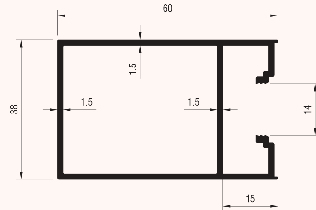
Profile Code : SD-1036 Unit Weight : 0.884 kg/m Perimeter : 280.5 mm
