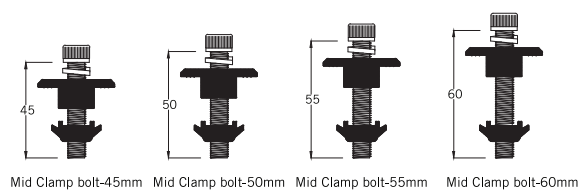
Mid Clamp bolt-45mm Mid Clamp bolt-50mm Mid Clamp bolt-55mm Mid Clamp bolt-60mm
