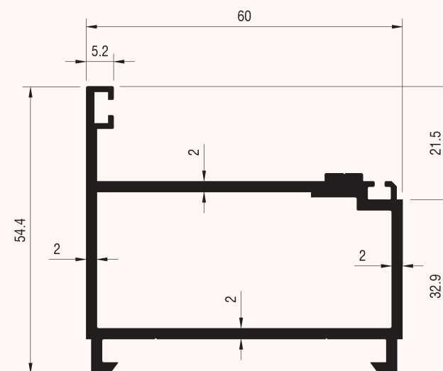
Profile Code : FD-6003 Unit Weight : 1.205 kg/m Perimeter : 284.2 mm
