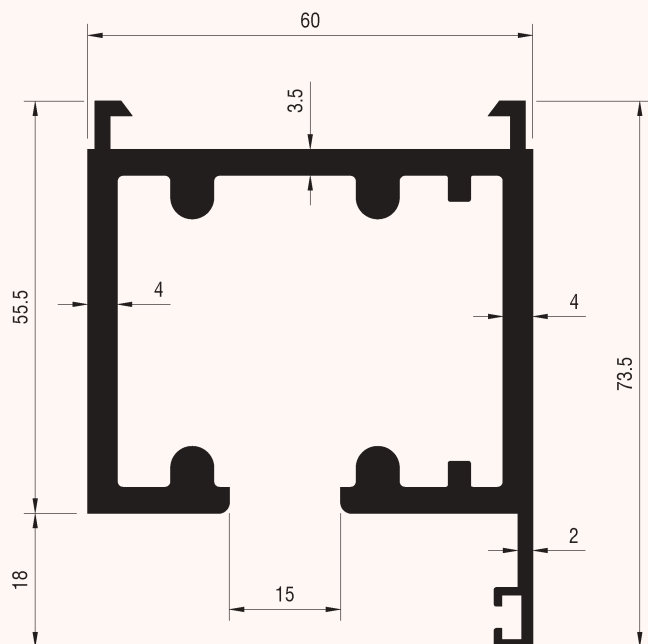
Profile Code : FD-6001 Unit Weight : 2.483 kg/m Perimeter : 517.5 mm
