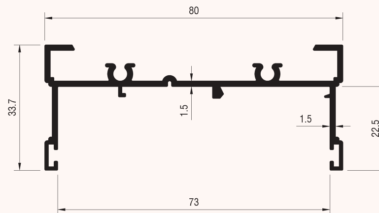
Profile Code : SW-8012 Unit Weight : 0.800 kg/m Perimeter : 404.9 mm
