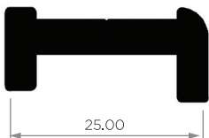
25,00 Profile Code - GS 1005 Linear Weight - 0.389 kg/m
