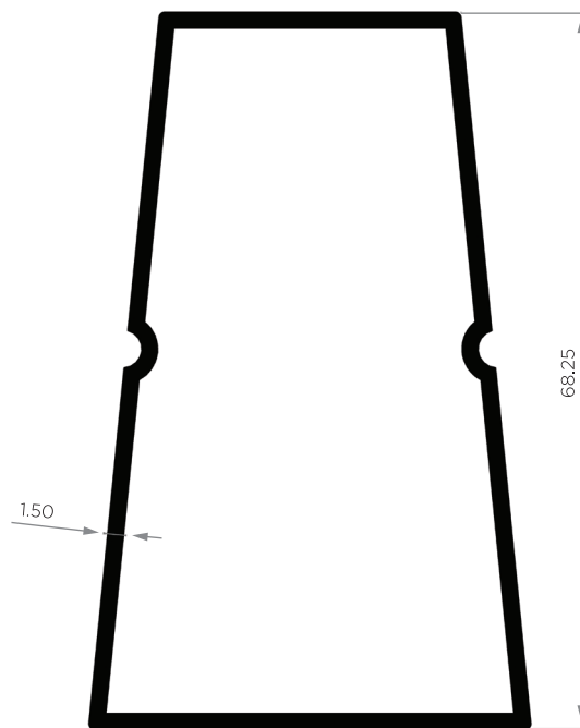
Profile Code - GS 1011 Linear Weight - 0.827 kg/m
