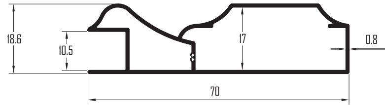
Profile No. : PC-2007 Est.Weight : 0.433 kg/m
