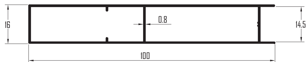
Profile No. : PC-2005 Est.Weight : 0.532 kg/m
