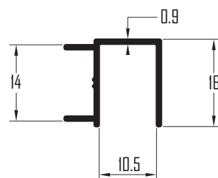
Profile No. : PC-2003 Est.Weight : 0.130 kg/m
