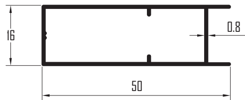
Profile No. : PC-2010 Est.Weight : 0.269 kg/m
