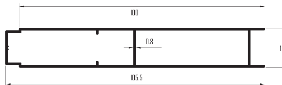
Profile No. : PC-2006 Est.Weight : 0.555 kg/m
