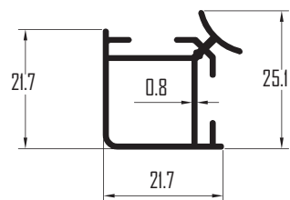
Profile No. : PC-2001 Est.Weight : 0.239 kg/m
