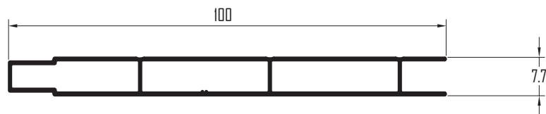
Profile No. : DD-6304 Est.Weight 0.425 kg/m
