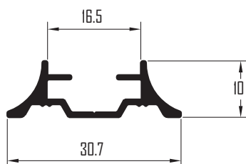
Profile No. : PC-2002 Est.Weight : 0.178 kg/m
