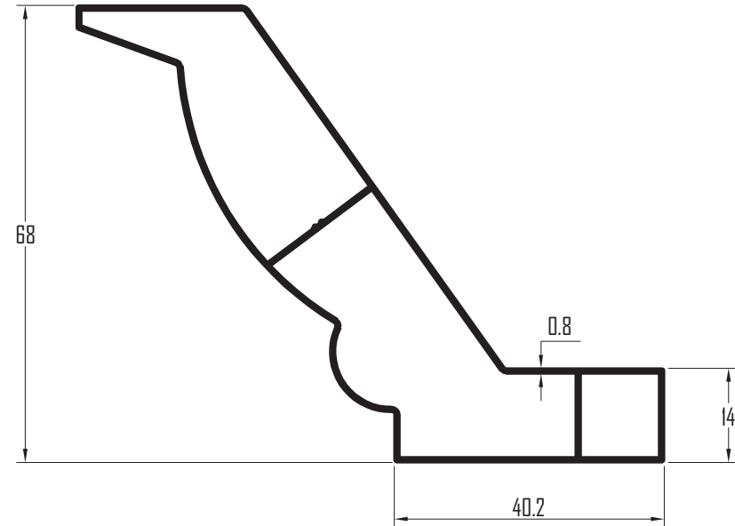
Profile No. : PC-2009 Est.Weight : 0.626 kg/m
