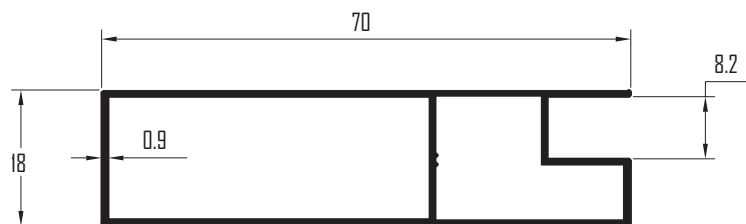
Profile No. : PC-1007 Est.Weight 0.486 kg/m
