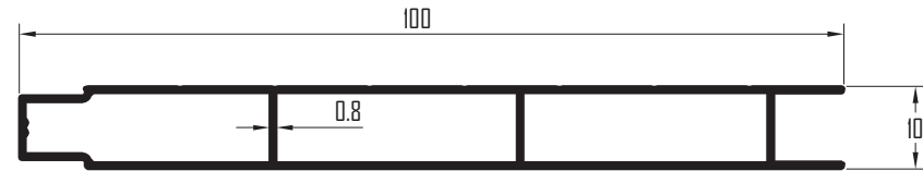
Profile No. : PC-2008 Est.Weight : 0.505 kg/m
