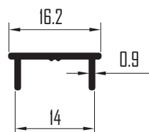
Profile No. : PC-2004 Est.Weight : 0.067 kg/m
